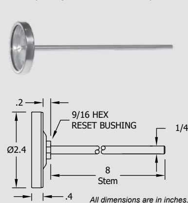
Lab Model HL with 2.4" Dial (with point - Model HLP)
