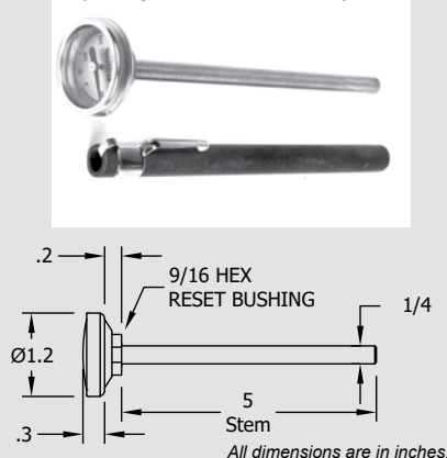
Lab Model QP with 1.2" Dial (with point - Model QPP)
