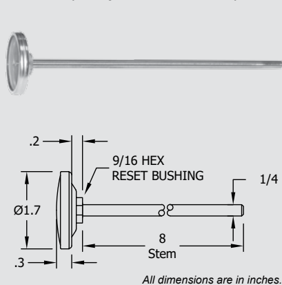
Lab Model GL with 1.7" Dial (with point - Model QLP)
