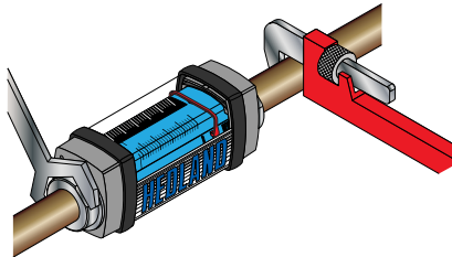
Figure 3: Installing meter
