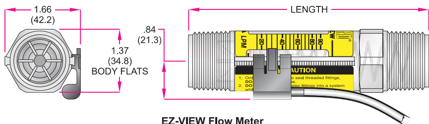
EZ-View Flow Meter (with Flow-Alert Reed Switch)
