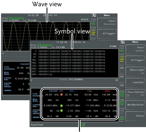
FSK demodulation measurements
