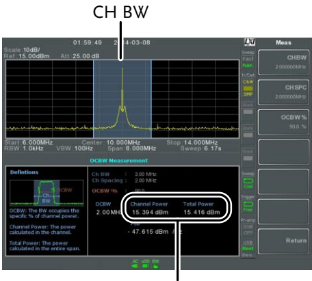
Channel power and total power results
