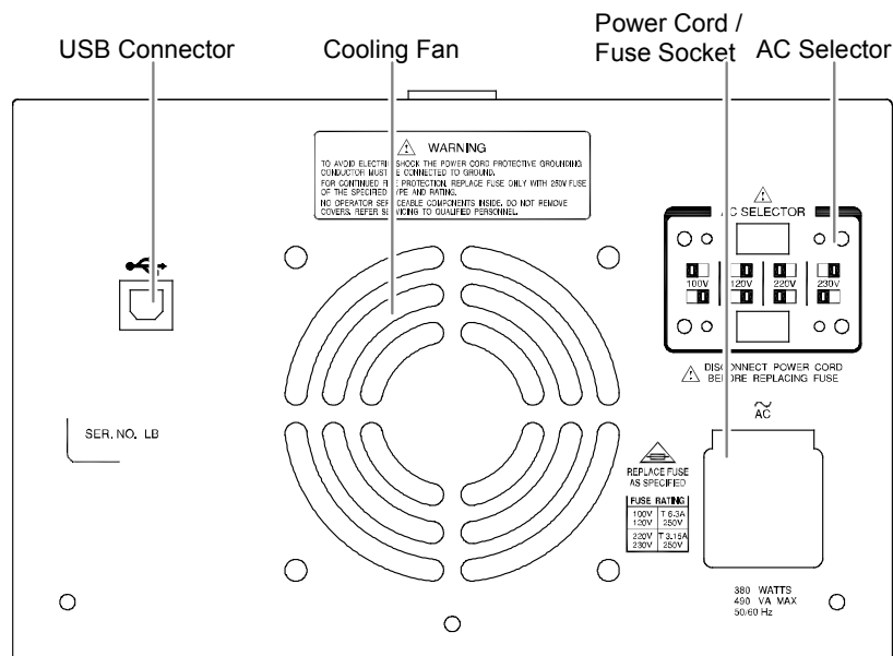
USB Connector
