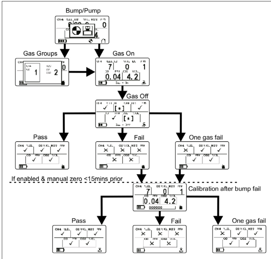
Figure 21: Gas test screen flow
