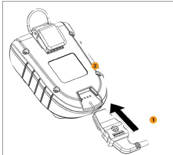
Figure 2: Charger connection
