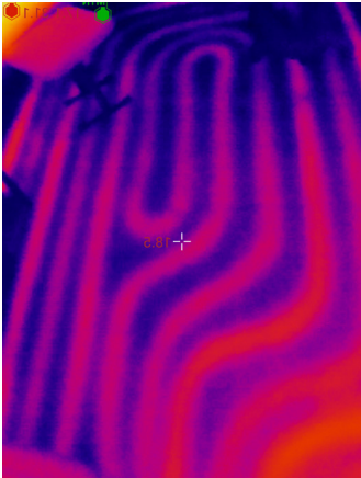
Floor heating
