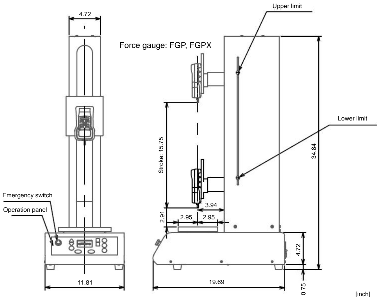
FGS-220VC
