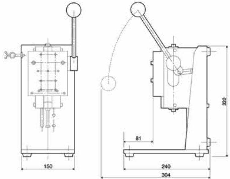
FGS-50S Dimensions in mm
