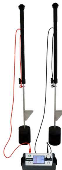
ESG NT2 set for voltage gradient method (step voltage method)
