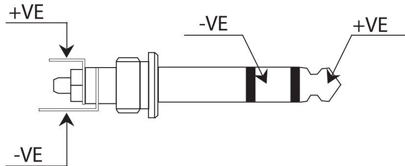
Figure 3 Jack Plug Wiring
