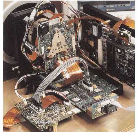
Figure 25.3 LEFT: Development of system electronics; RIGHT: Testing of an FPA detector
