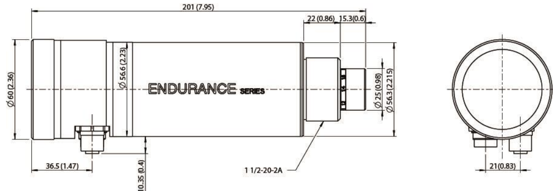
Figure 3: Dimensions of Endurance® Sensor
