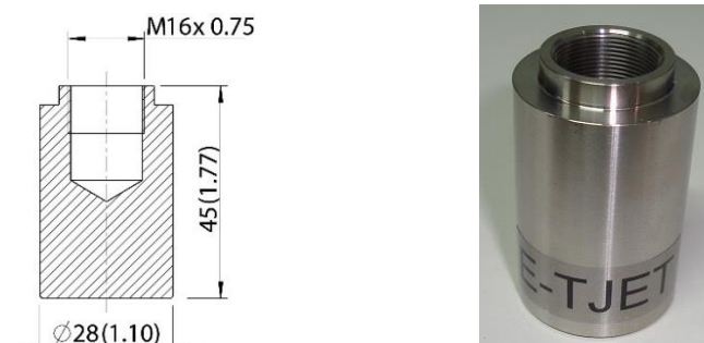
Figure 79: Drawing and picture of the extraction tool (E-TJET)
