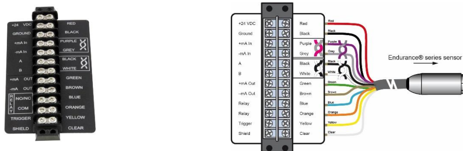
Figure 44: Endurance® Terminal Block (E-TB) with wire color assignment
