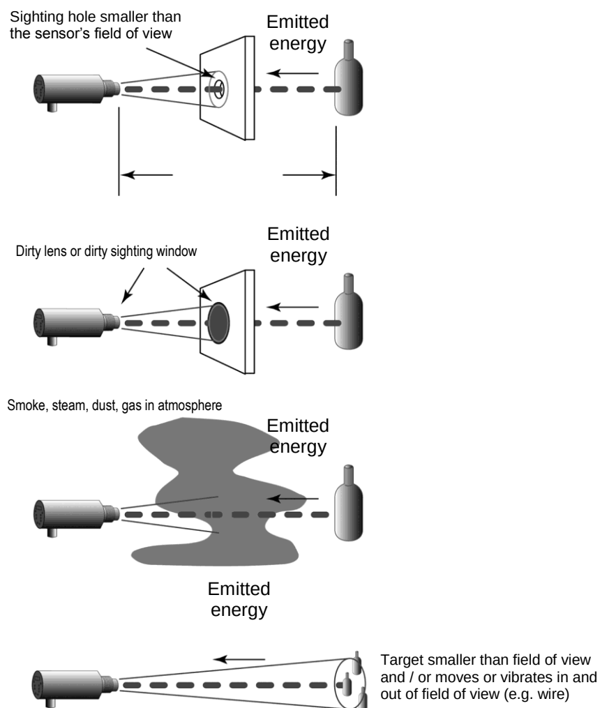
Figure 6: Sensor Placement in 2-Color Mode
