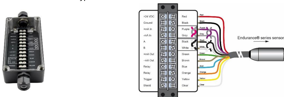
Figure 45: Endurance® Terminal Block in a NEMA 4 Enclosure (E-TBN4)
