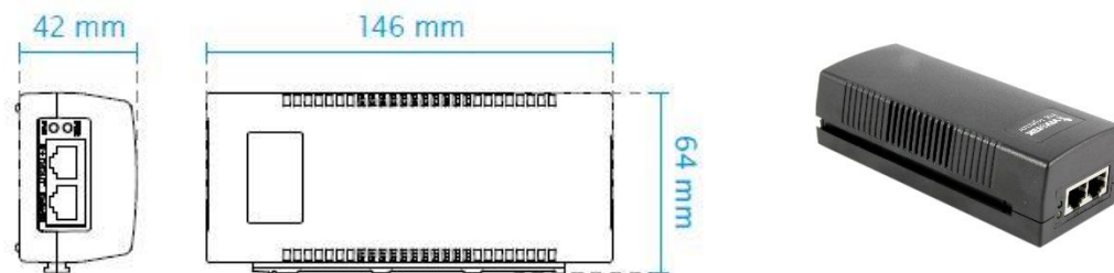
Figure 48: PoE Injector to provides power over a single Ethernet hub (E-POE)
