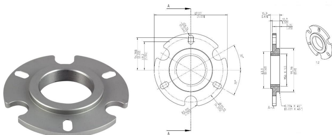
Figure 71: Mounting flange (E-MF-7)
