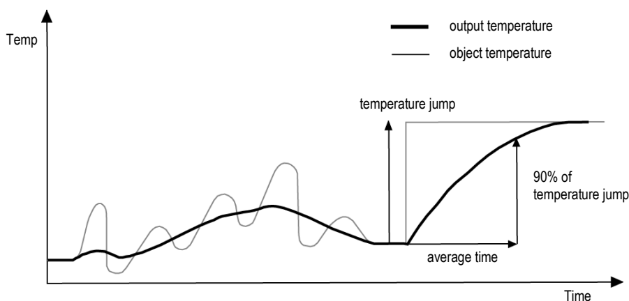
Figure 26: Averaging
