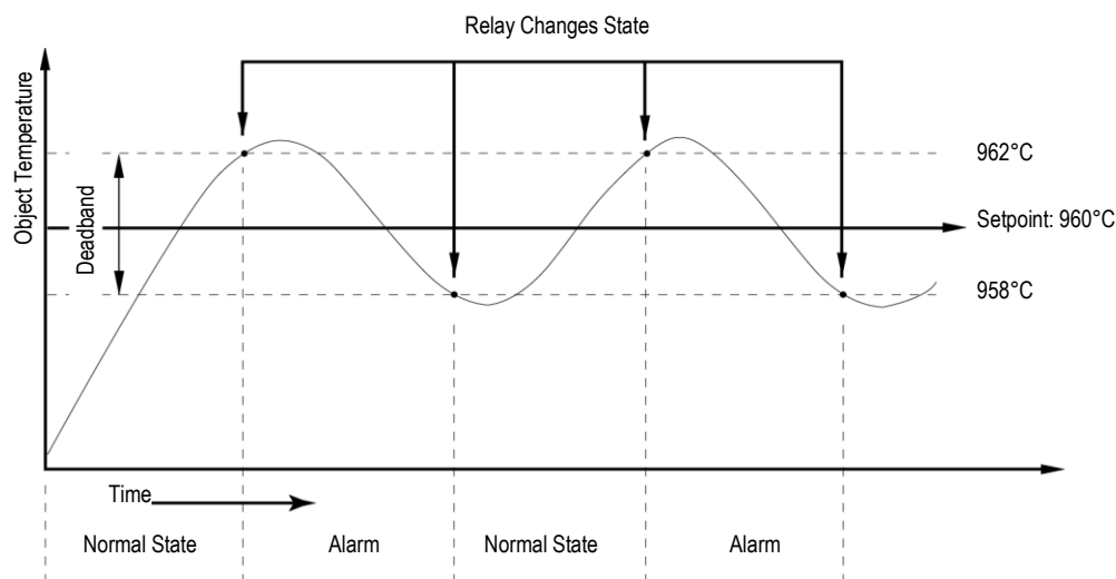
Figure 34: Deadband Example
