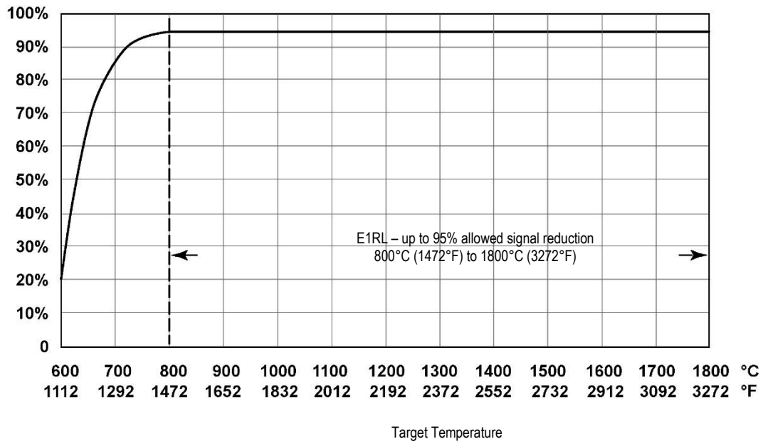
Figure 76: Model E1RL Percentage of Allowed Signal Reduction
