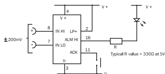
Using an external LED as a high alarm and a switch to acknowledge the alarm (to stop it flashing) Typical R value = 330Ω at 5V
