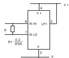
Measuring current. Supply MUST be isolated R = \frac{0.2}{I_{FSR}}
