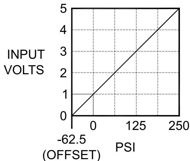
Figure 2.5 Linear Scaling
