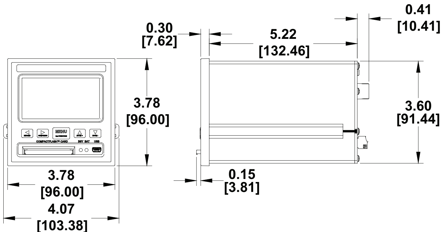
Figure 2.1 Recorder Dimensions
