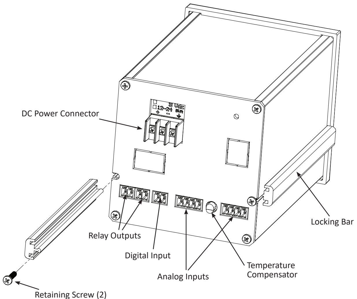
Figure 2.2 Rear View — Installation
