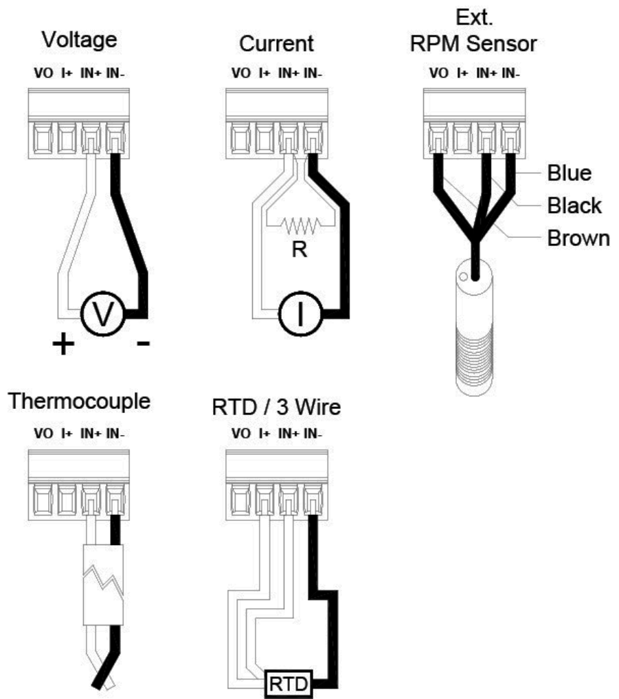
Figure 2.4 Connection Detail
