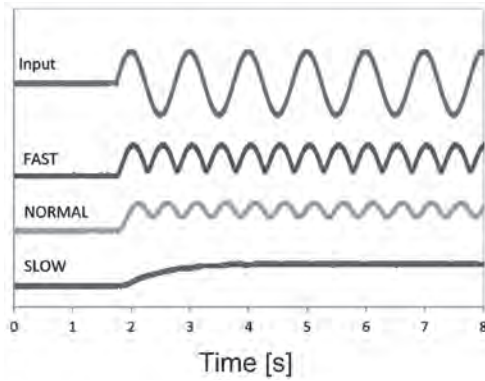
Fig. 24. RMS output with 1 Hz input.
