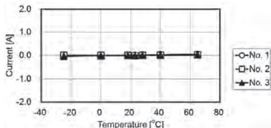
Fig. 13. Example CT7731 offset-temperature characteristics.
