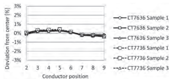
Fig. 18. Example 600 A conductor position characteristics.
