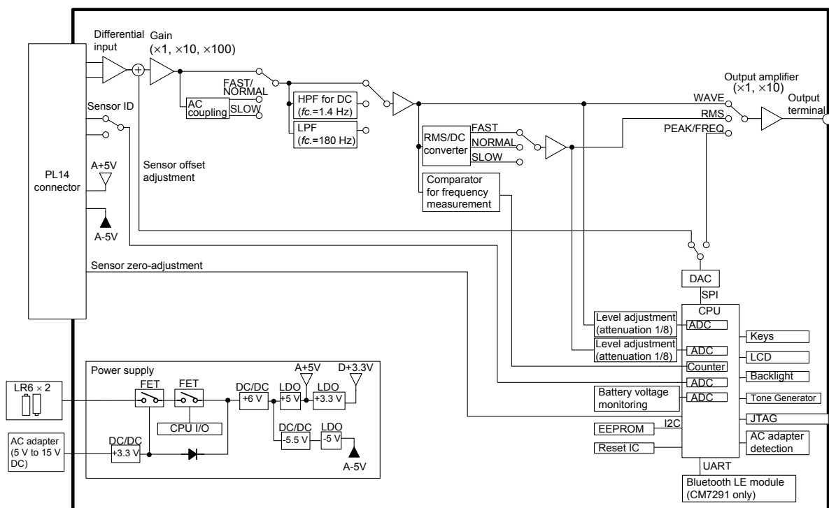
Fig. 3. Block diagram (CM7290/CM7291).
