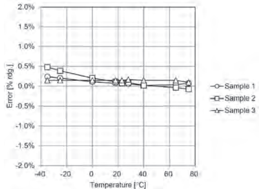
Fig. 23. Temperature characteristics (AC 600.0 mV range, 540 mV/55 Hz input).
