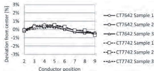
Fig. 19. Example 2000 A conductor position characteristics.
