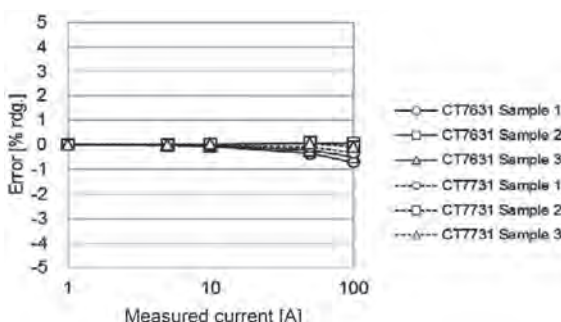
Fig. 7. Example 100 A sensor amplitude-accuracy characteristics.
