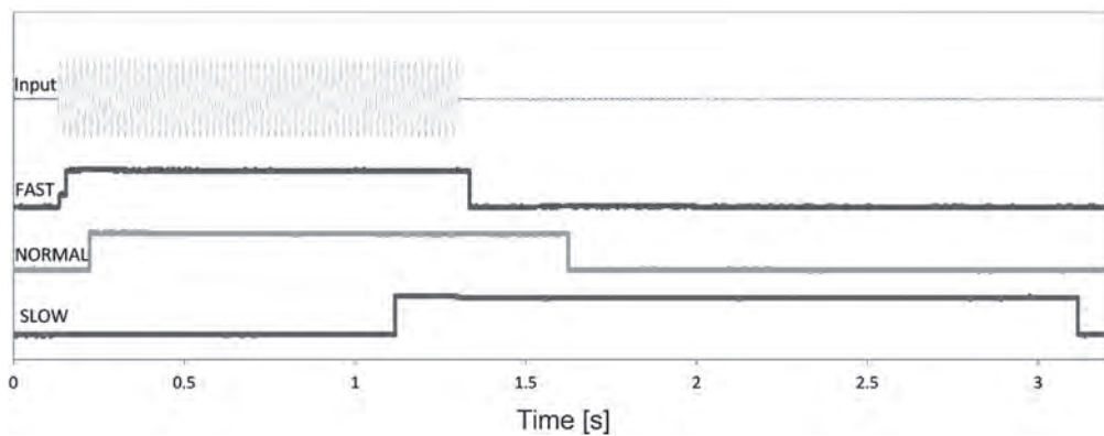
Fig. 28. PEAK output with 50 Hz input.
