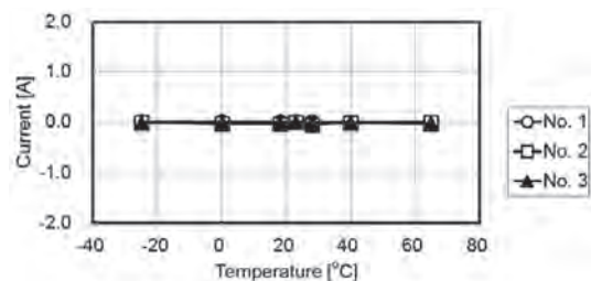
Fig. 14. Example CT7736 offset-temperature characteristics.
