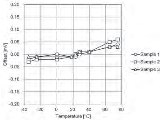
Fig. 20. Temperature characteristics (DC 60.00 mV range, no input).
