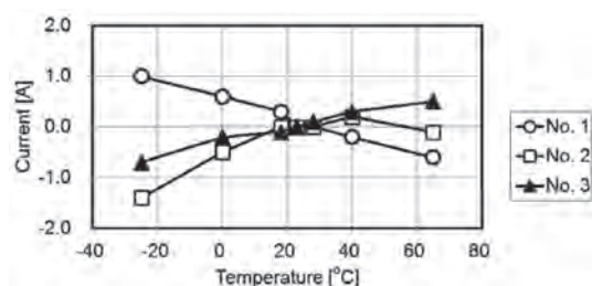
Fig. 12. Example CT7642 offset-temperature characteristics.
