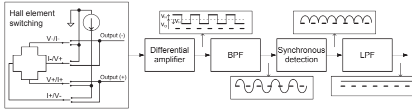
Fig. 2. Block diagram (CT7731/CT7736/CT7742).
