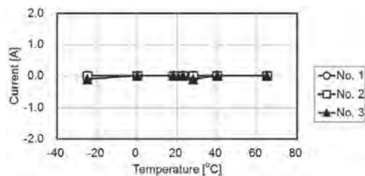
Fig. 15. Example CT7742 offset-temperature characteristics.
