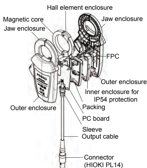
Fig. 4. CT7636/CT7736 construction.
