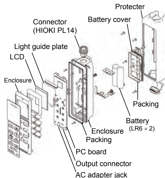
Fig. 5. CM7290/CM7291 construction.
