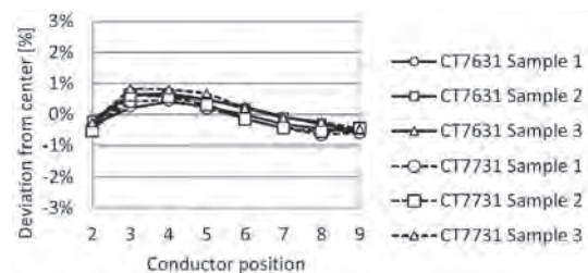
Fig. 17. Example 100 A conductor position characteristics.
