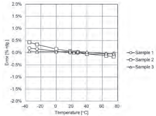
Fig. 22. Temperature characteristics (AC 60.00 mV range, 54 mV/55 Hz input).
