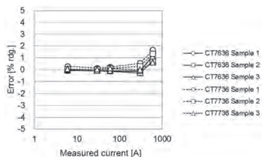
Fig. 8. Example 600 A sensor amplitude-accuracy characteristics.
