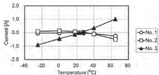
Fig. 11. Example CT7636 offset-temperature characteristics.
