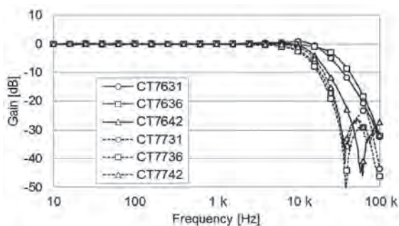
Fig. 6. Example sensor frequency characteristics.
