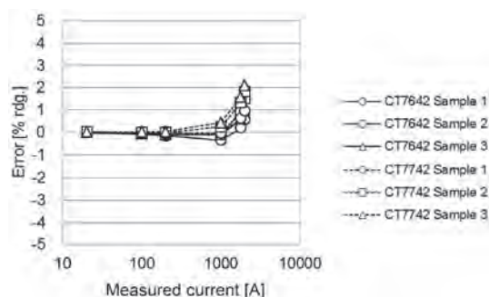
Fig. 9. Example 2000 A sensor amplitude-accuracy characteristics.
