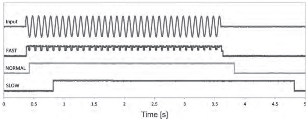
Fig. 27. PEAK output with 10 Hz input.
