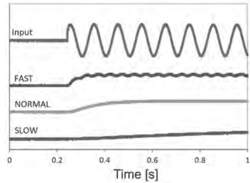
Fig. 25. RMS output with 10 Hz input.
