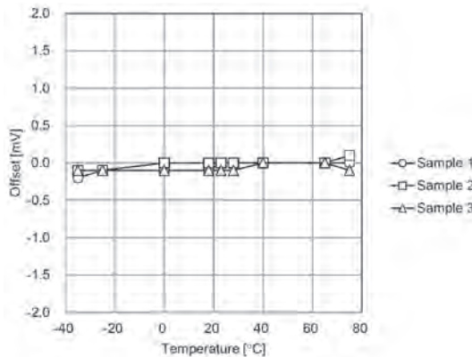
Fig. 21. Temperature characteristics (DC 600.0 mV range, no input).
