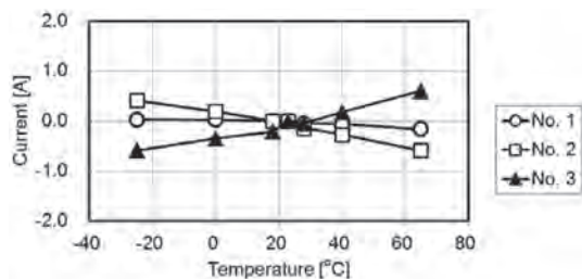
Fig. 10. Example CT7631 offset-temperature characteristics.
