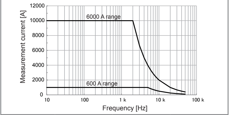
Frequency derating (continuous, design values)
