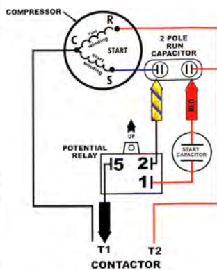
2 POLE RUN CAPACITOR
