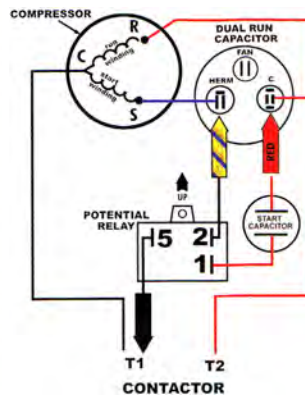
DUAL RUN CAPACITOR
