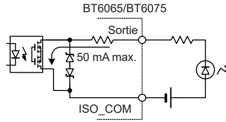
Raccordement à la LED
