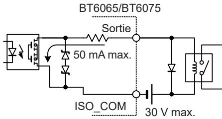
Raccordement au relais
