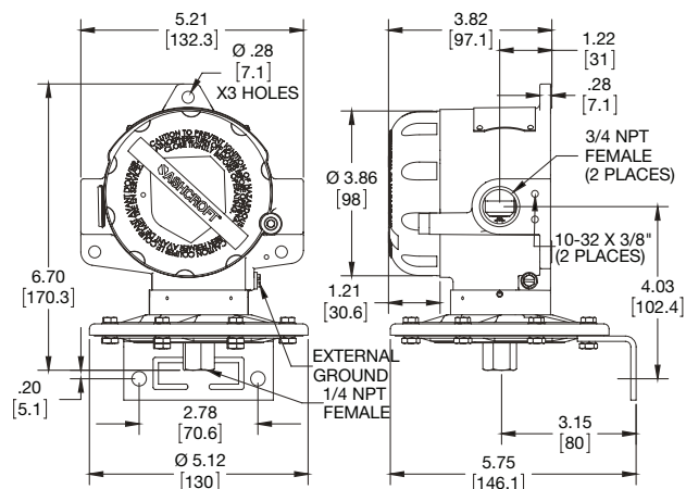
Pressure switch – inches of water ranges
