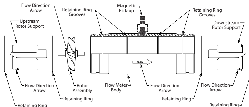
Figure 9: Component positions for B111-140 and B111-200
