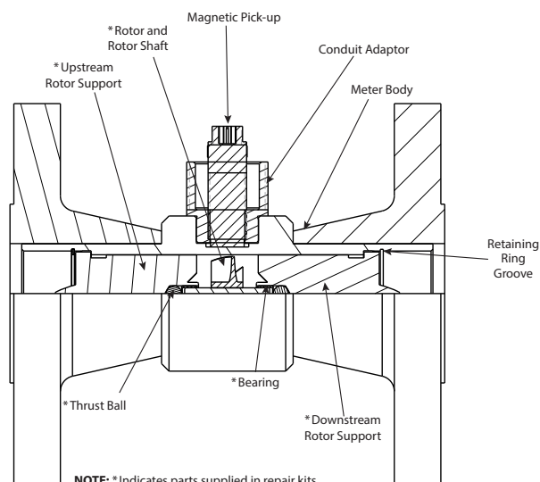
Figure 1: Meter components
