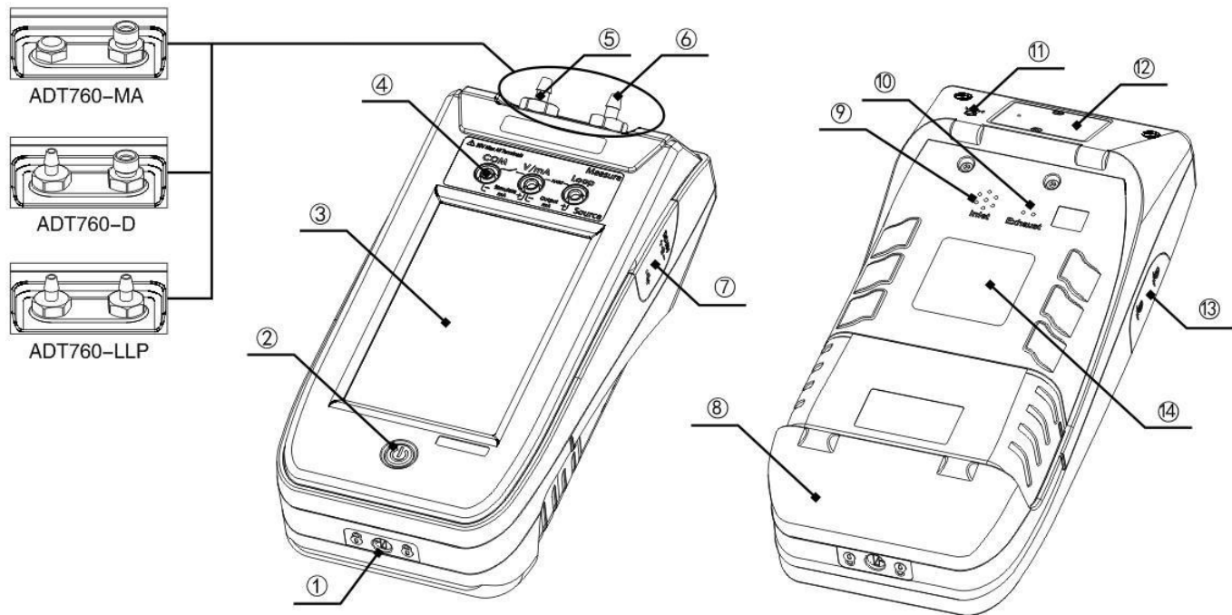
Figure 1 Basic Structure
