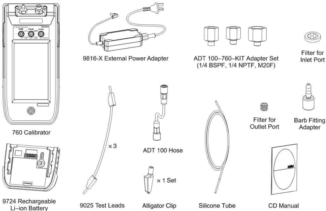
Figure 2 Standard Equipment
