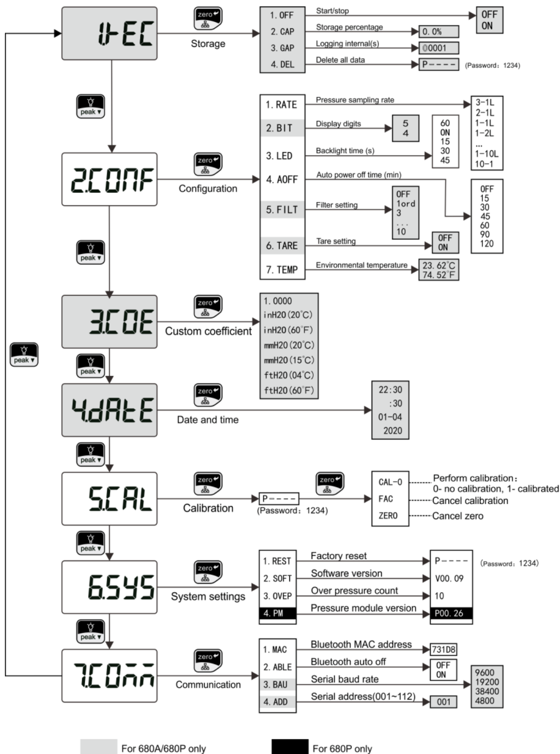
Menu structure
