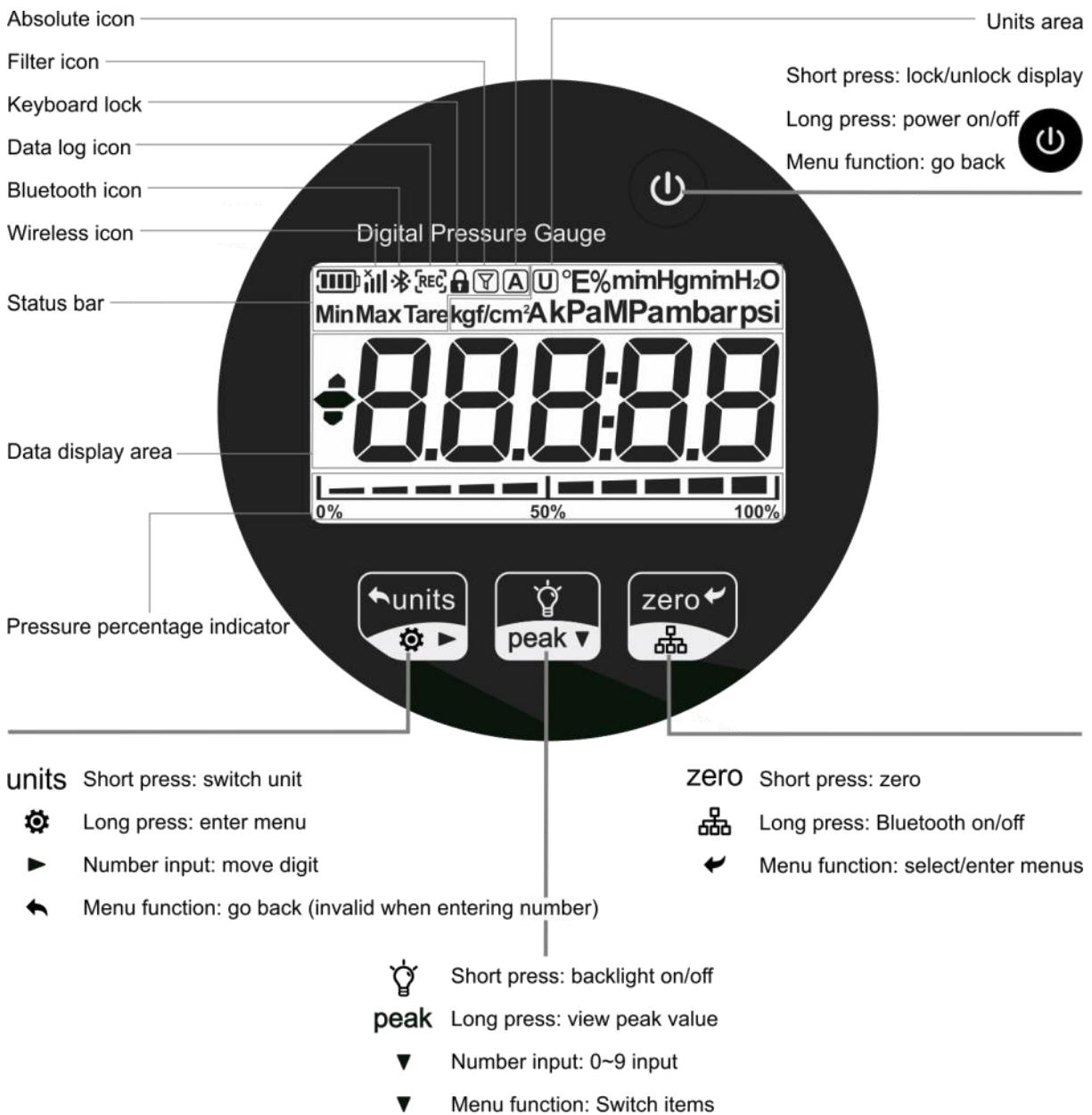
Display and buttons description
