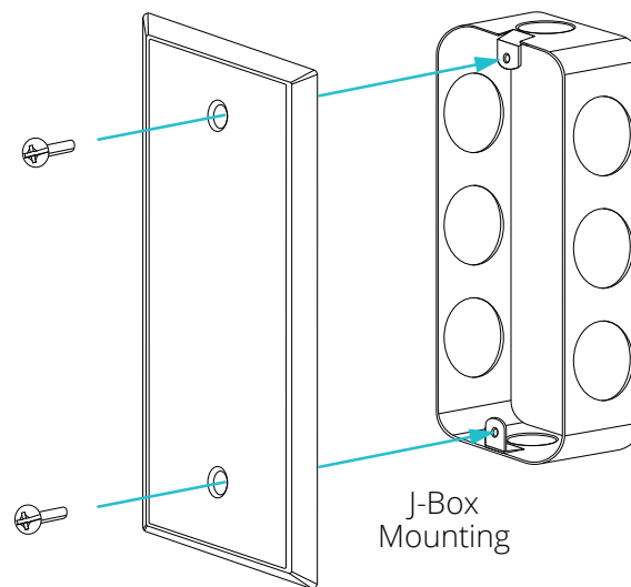
Figure 5 AcuTEMS WP Junction Box Mounting
