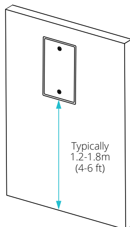
Figure 2 AcuTEMS WP Typical Mounting Location
