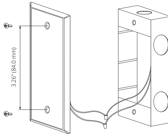
Figure 3 AcuTEMS WP Flying Lead Connection
