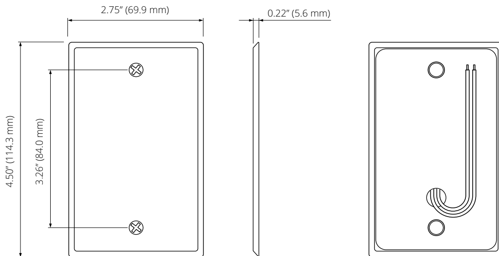
Figure 1 AcuTEMS WP Front and Side Views
