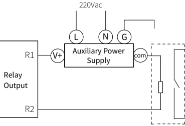
Relay output
