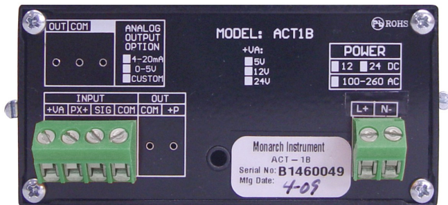
Rear Panel
