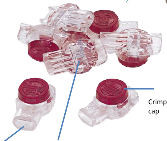
Internal IDC bus bar
