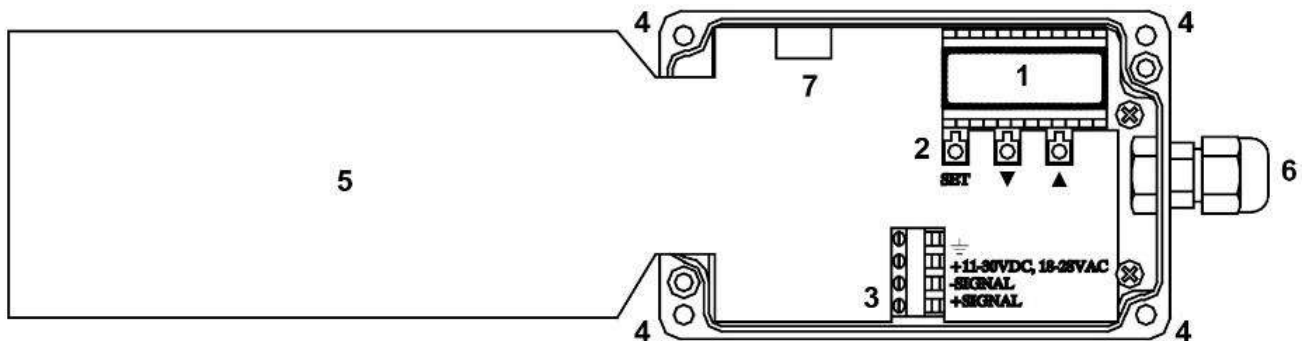
Figure 2: Inside of Electronic Enclosure
