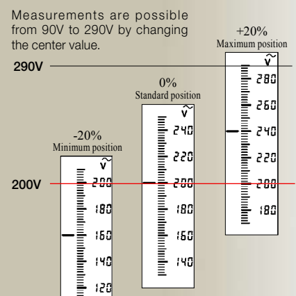
Example of a level display for the 200V range
