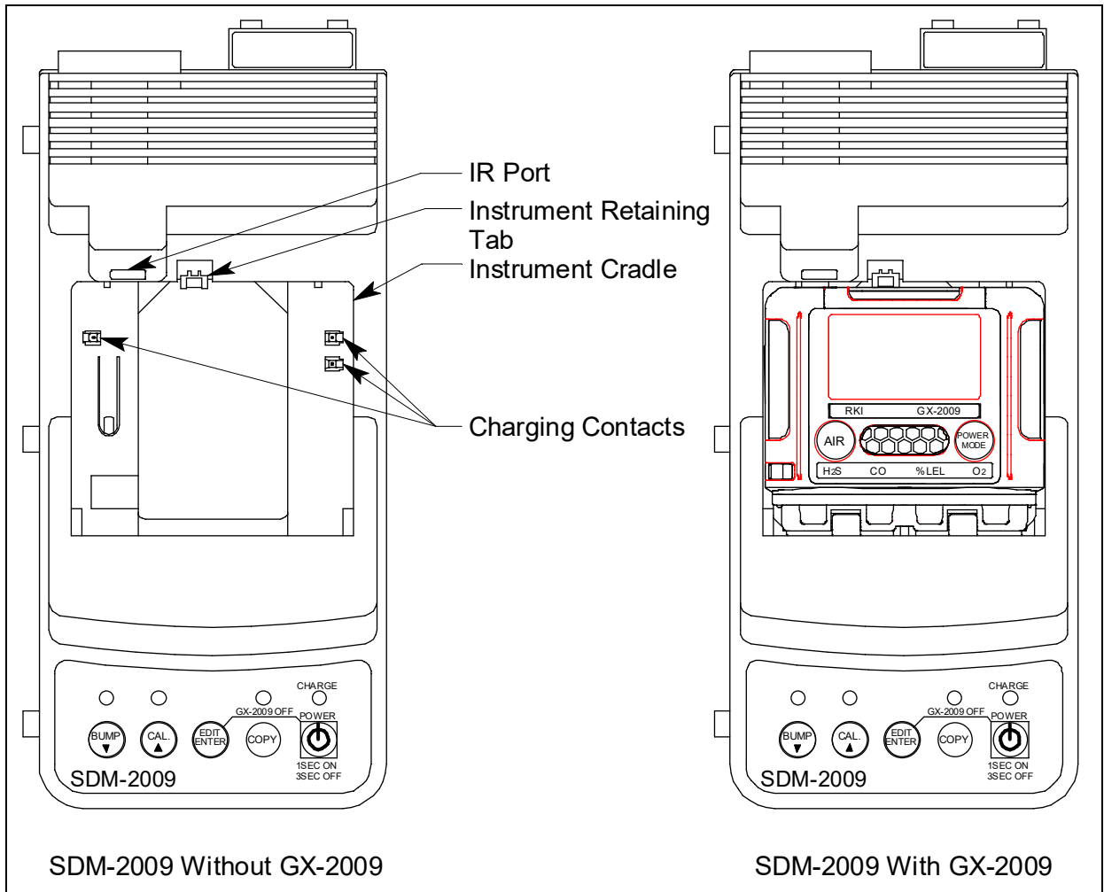
Figure 7: Instrument Cradle
