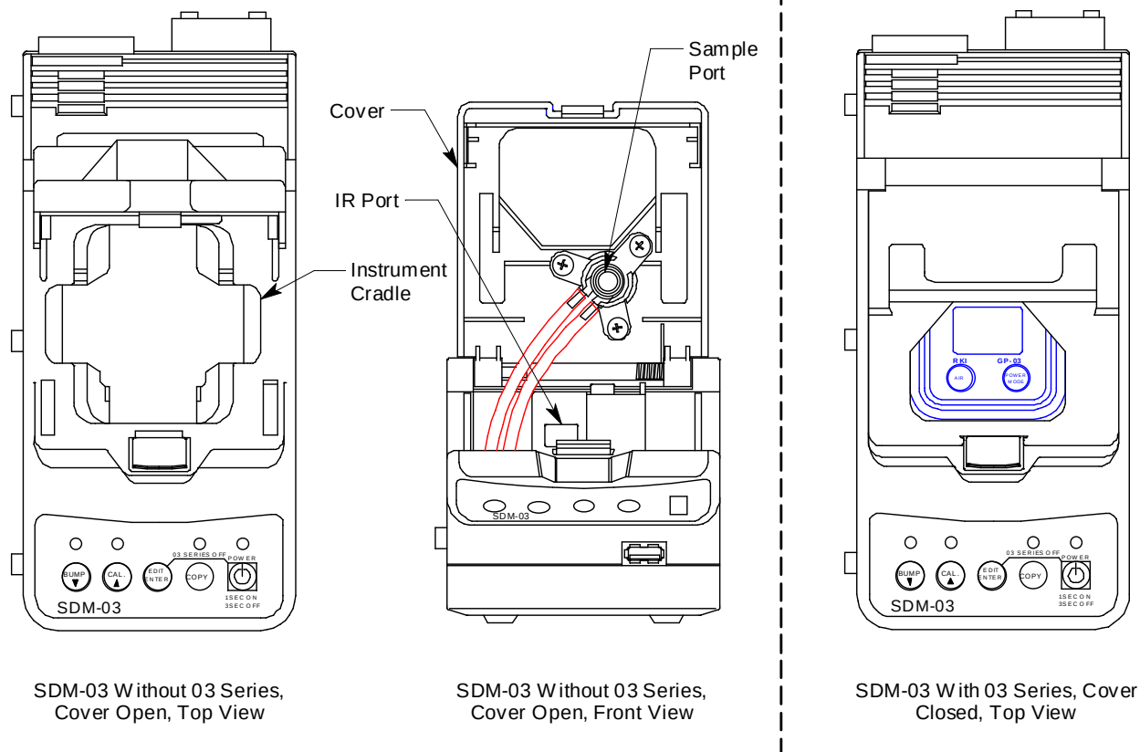
Figure 7: Instrument Cradle
