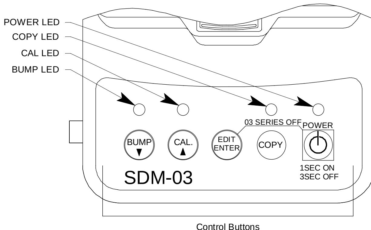
Figure 9: Control Panel
