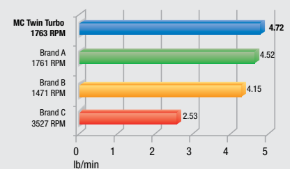
Vapor Recovery (Out) lb/min • Temperature: 79 to 82°F / Refrigerant: R134a
