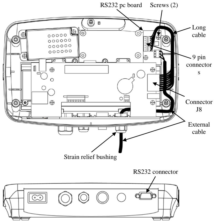
Figure 2.3. T51P, T71P
