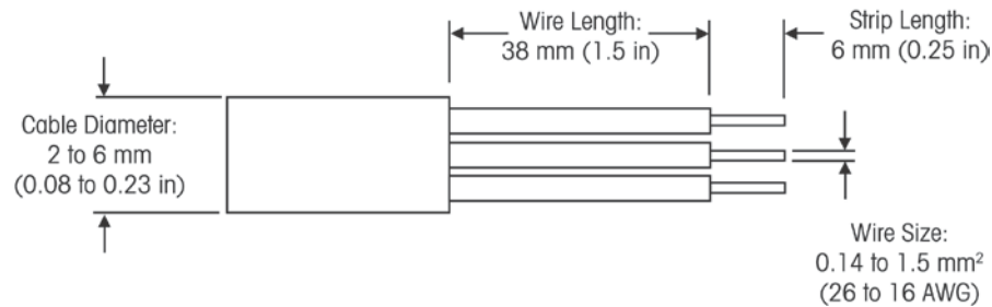
Figure 2.1 Wire Preparation
