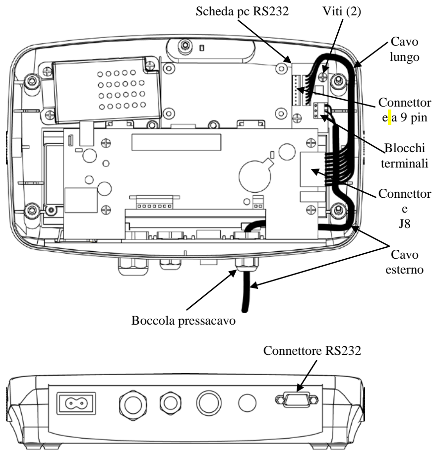
Figura 2.3. T51P, T71P
