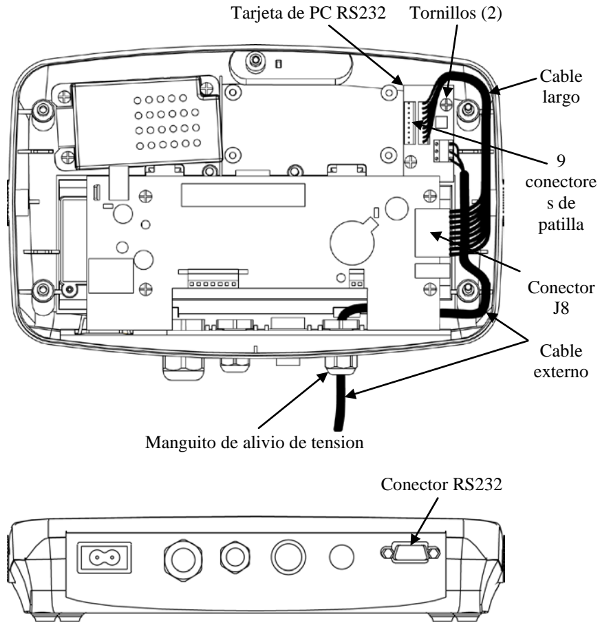
Figura 2.3. T51P, T71P
