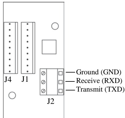
Figure 2.2 RS232 Connections
