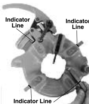
Figure 12 – Inserting Dies
