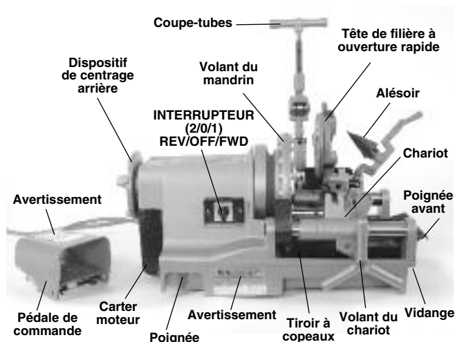
Figure 1 – Fileteuse 300 Compact
