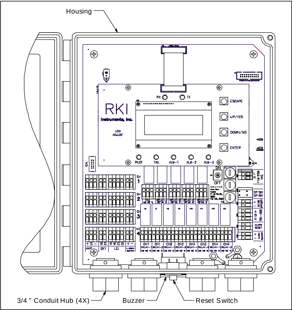
Figure 1: External Component Location
