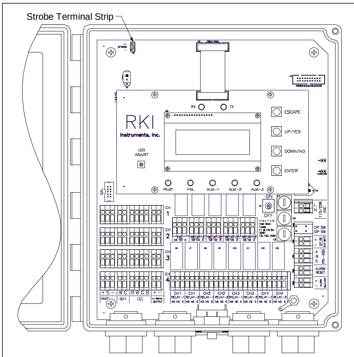
Figure 6: Strobe Terminal Strip Location
