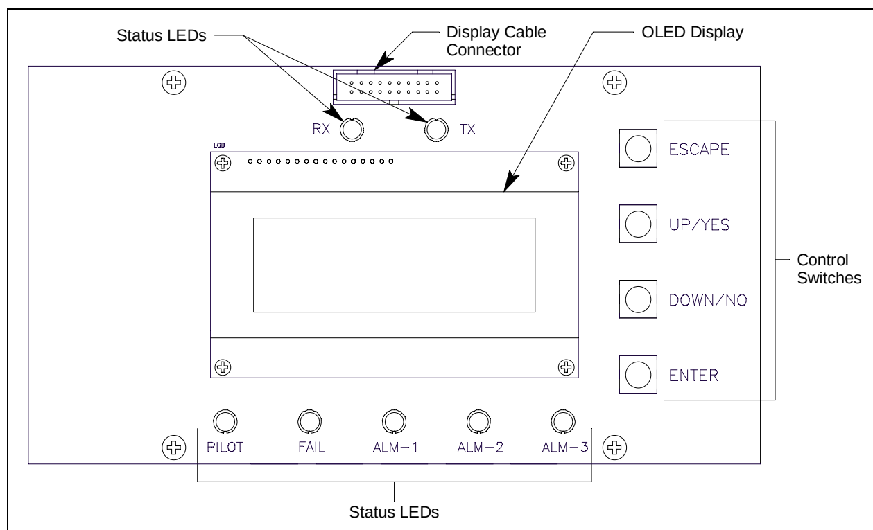
Figure 3: Control PCB Component Location
