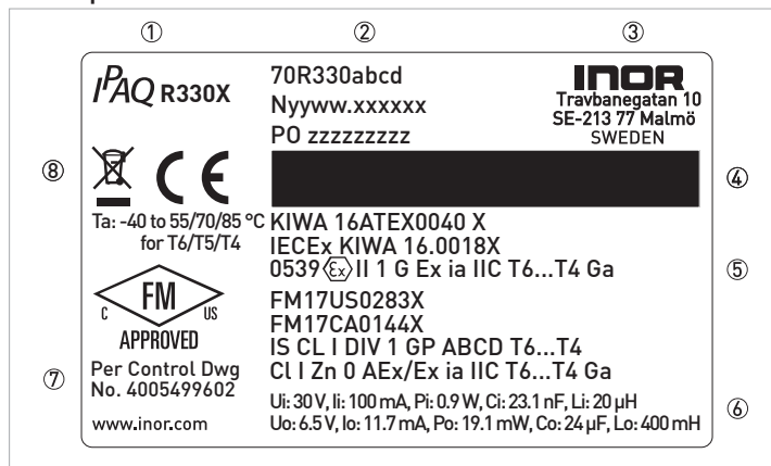
Figure 2-6: Example for nameplate
