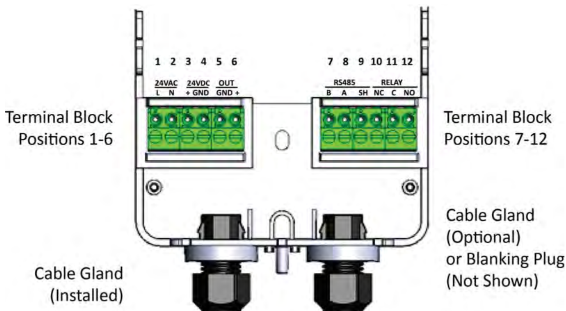
Figure 7. Terminal Blocks and Cable Glands
