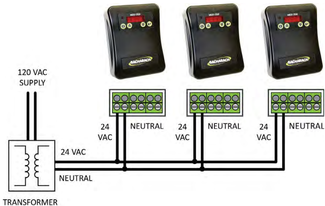
Figure 9. Maintaining Neutral Polarity
