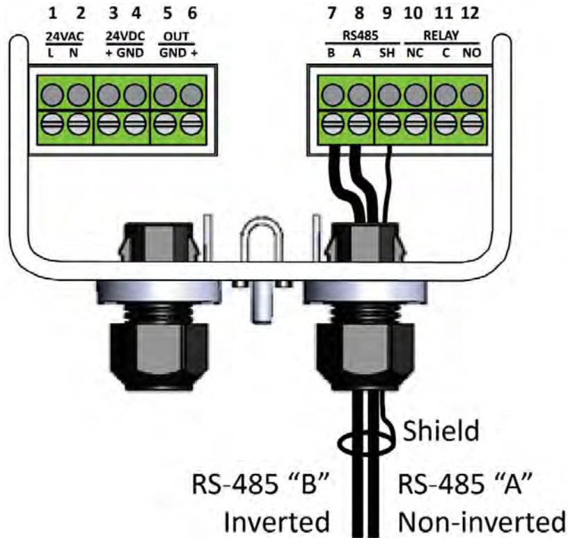
Figure 12. Modbus Network Wiring
