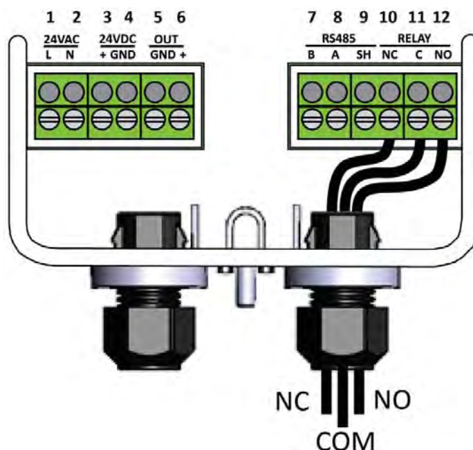
Figure 11. Sample Relay Output Wiring
