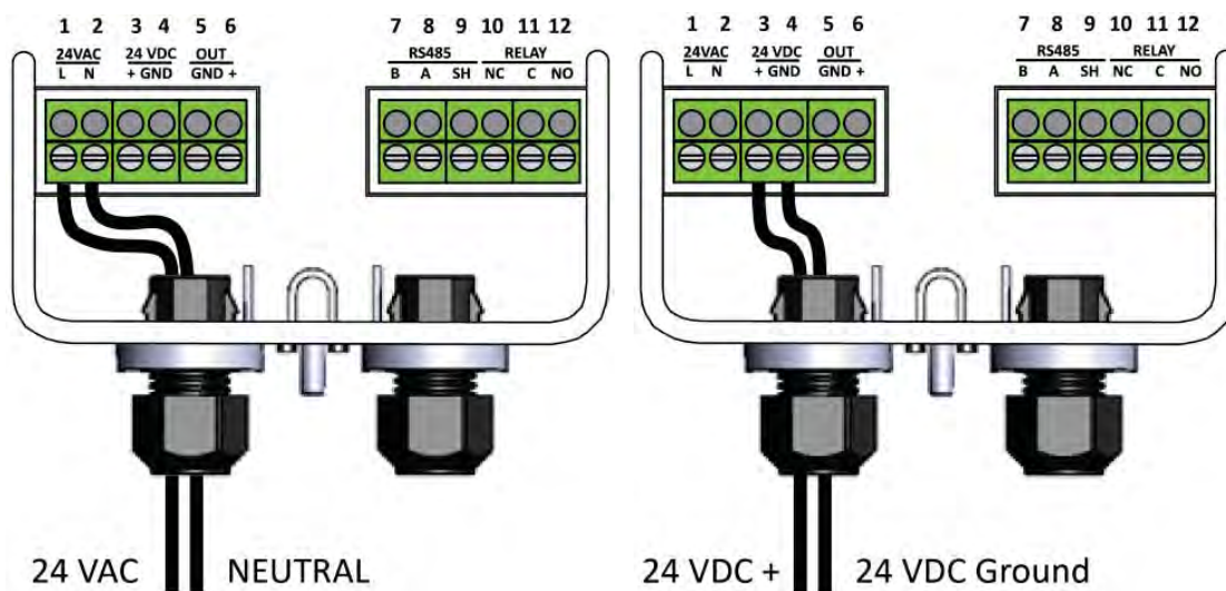
Figure 8. Supply Power Wiring Options
