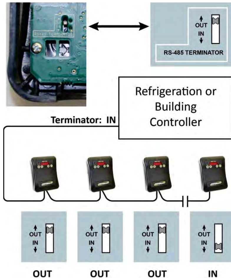
Figure 13. Setting Network Termination Resistors
