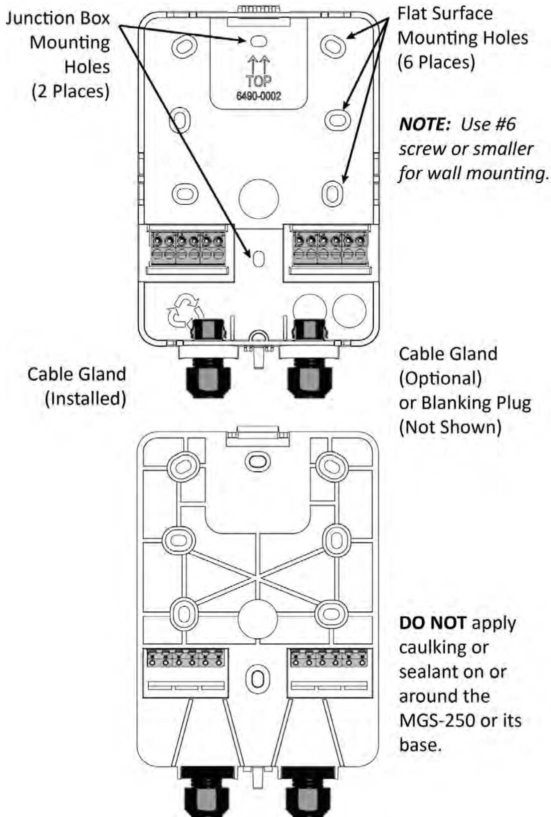
Figure 6. Front and Back Views of MGS-250 Base
