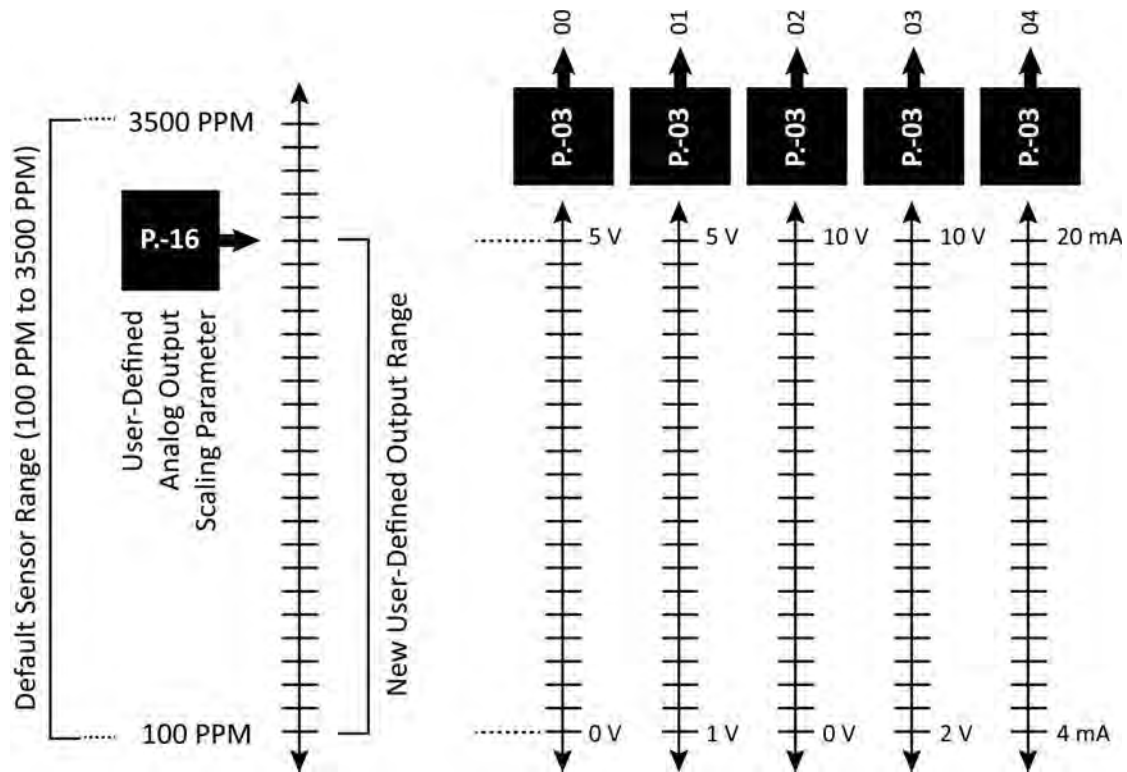
Figure 15. Analog Output Scaling Options
