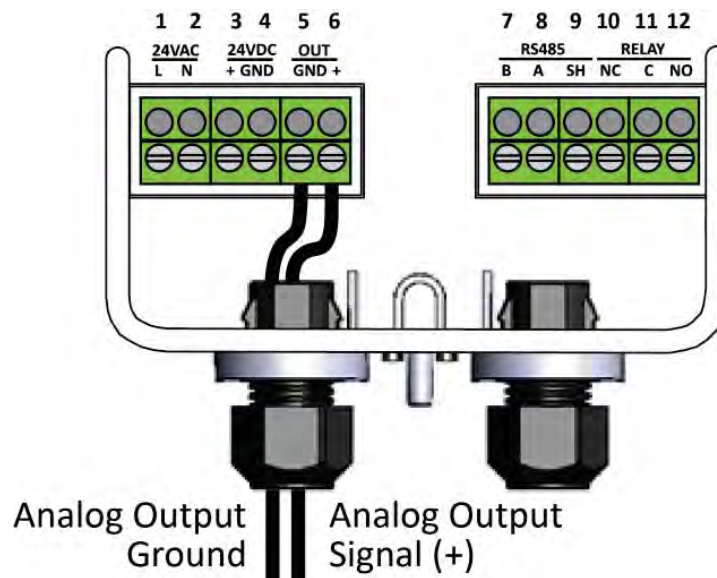
Figure 10. Analog Output Wiring
