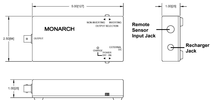
SPSR-IM Dimensions
