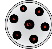
Multi-hole M02 (ATC-156/320/650 A/B / ITC-320/650 A)
