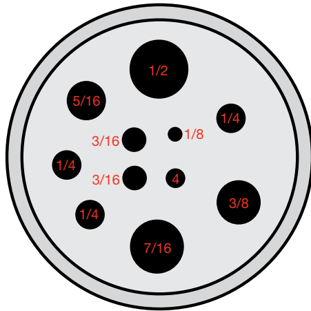
Multi-hole M02 (ATC-140/250 A/B)
