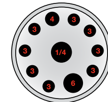
Multi-hole M03 (ATC-156/320/650 A/B / ITC-320/650 A)
