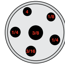
Multi-hole M06 (ATC-125 A/B)
