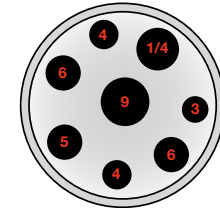
Multi-hole M04 (ATC-156/320/650 A/B / ITC-320/650 A)
