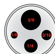
Multi-hole type 2 (CTC/MTC-320 A / 650 A)
