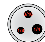
Multi-hole type 2 (CTC/MTC-140 A)
