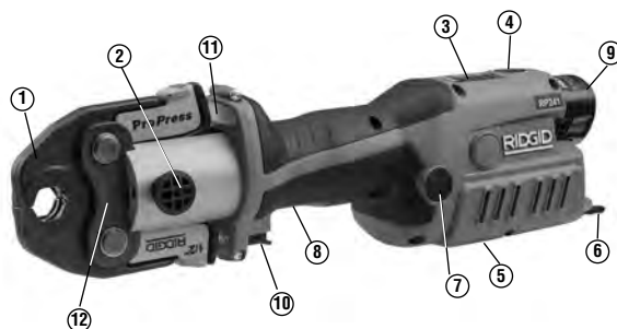
Figure 2 – RIDGID RP 241 Press Tool and Compact Series Jaw
