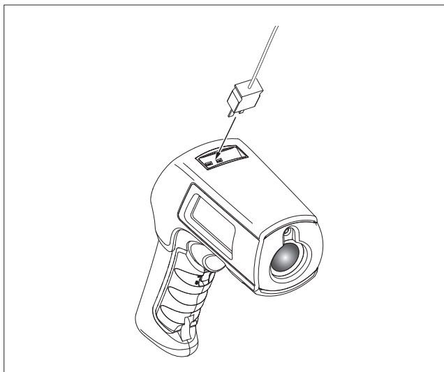
Figure 7. Thermocouple Connection
