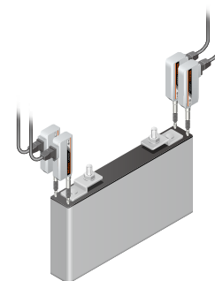
Battery flatness measurement
