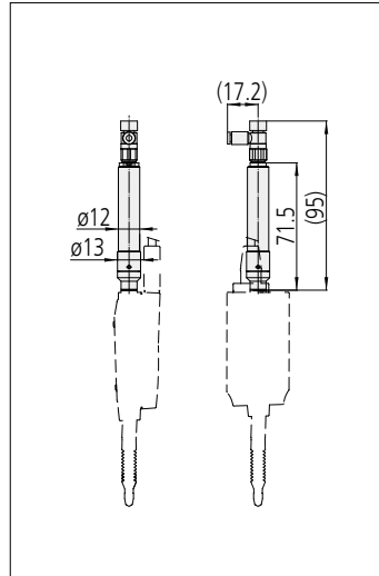
Air lifting unit LGS
