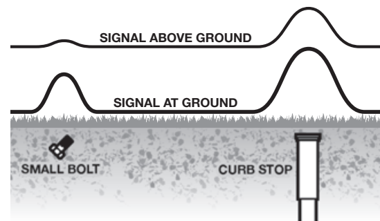
Figure 6 – Raising the Locator Minimizes Unwanted Signals
