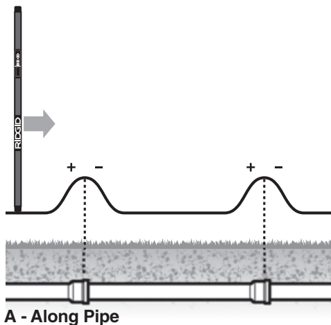
Figure 8 – Signal Patterns from Cast-Iron Pipe
