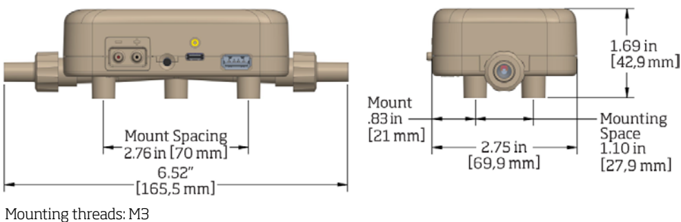
5200 Series Dimensions
