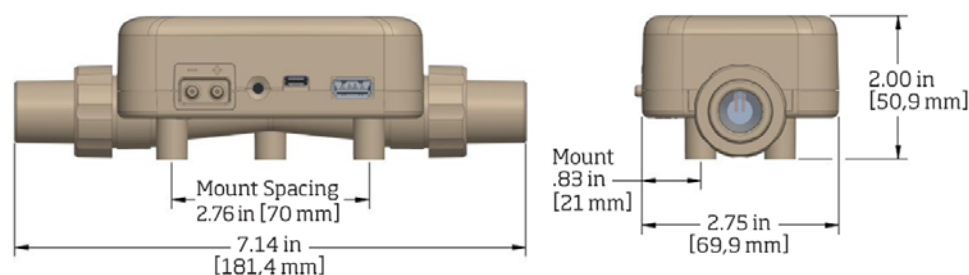
5300 Series Dimensions
