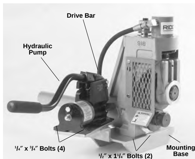
Figure 7 – 918 Roll Groover on 535 Threading Machine Mounting Base
