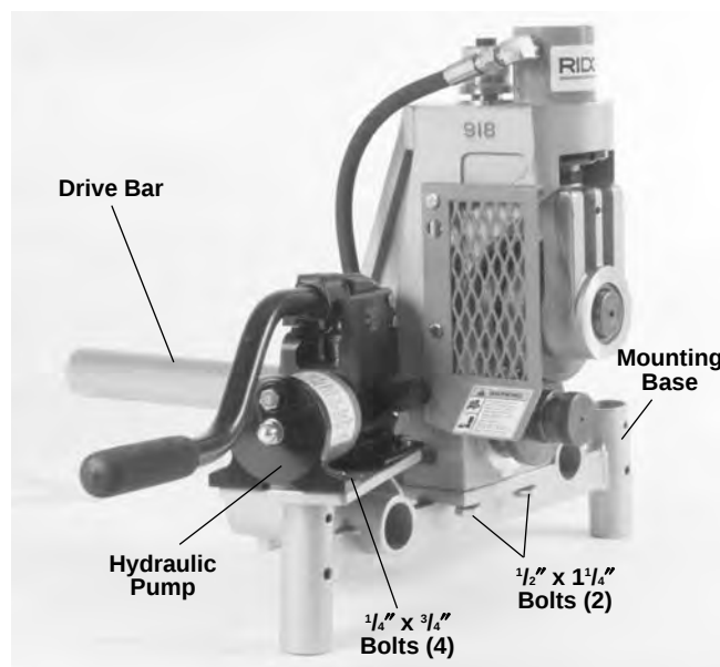
Figure 3 – 918 Heavy Duty Roll Groover on 1822 Mounting Base
