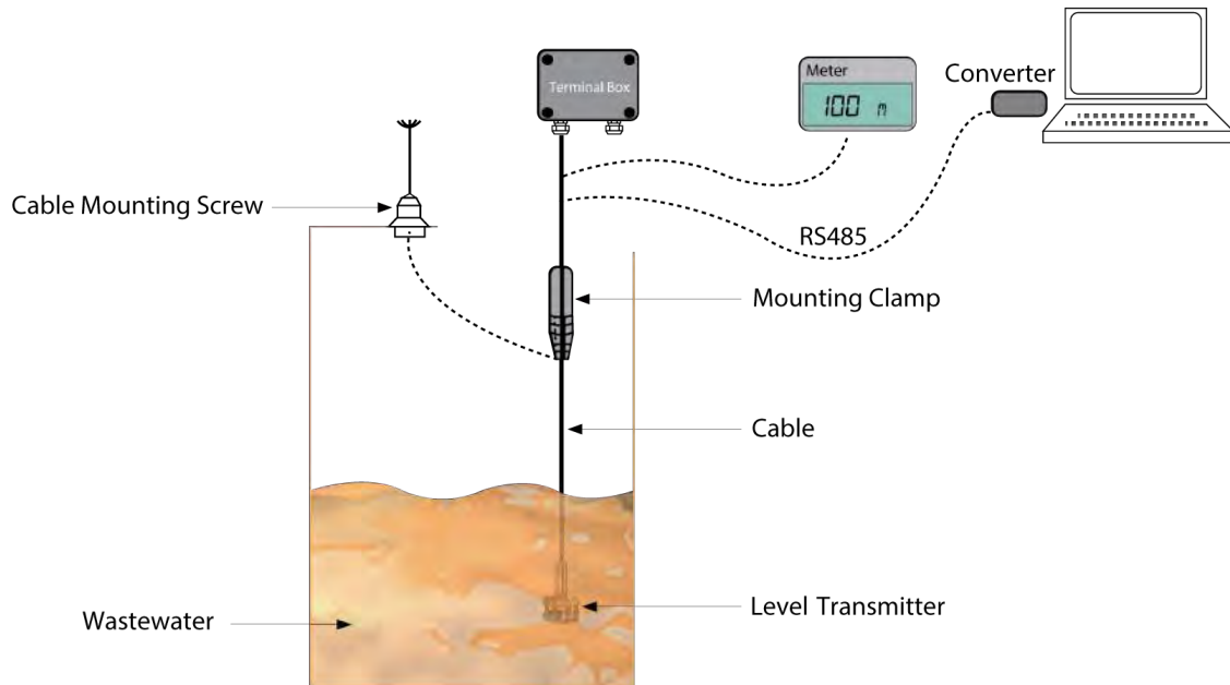
Fig.2. Mounting the transmitter
