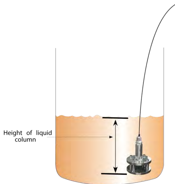
Fig.1. Measuring Principle
