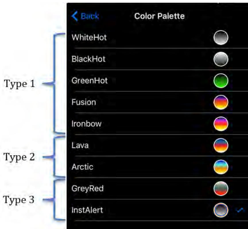
Figure 11. Color Palettes
