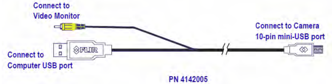
Figure 2. Bench Cable
